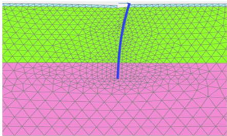
Fig. 3. Horizontal displacement of soil under load Q_x = 2.5 tons
