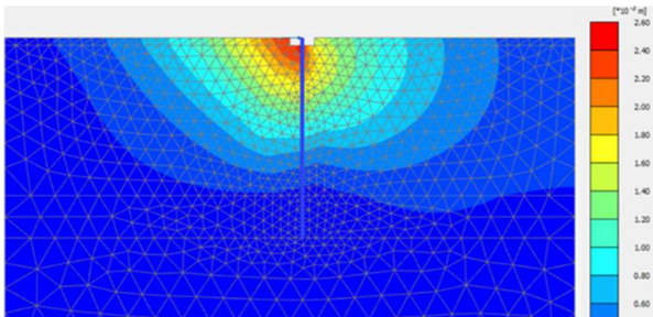
Fig 5. Maximum horizontal load. Q_x = 15.0 tons
