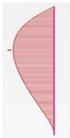
Bending moment diagram M_x = 3.27 tons·m
