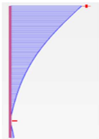
Diagram of horizontal displacement, U_x = 4.2 mm
