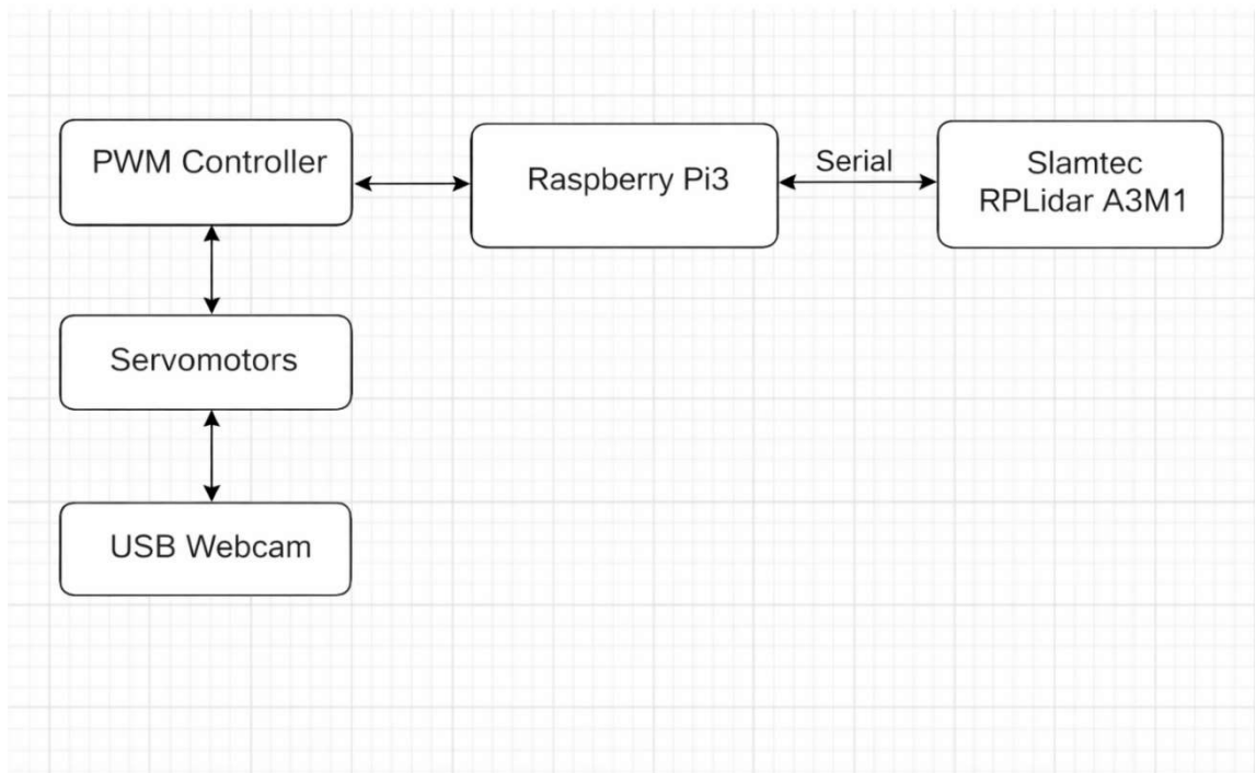
Fig. 4. – Diagram of interaction of components of the MRK
